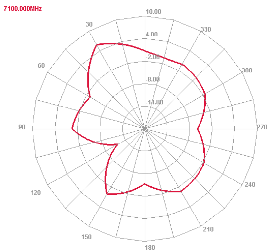
E plane
